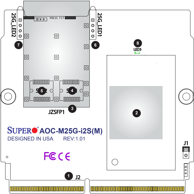
AOC-M25G-i2S(M) Layout
