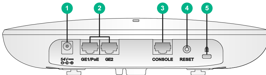
Figure 19 Ports on the H3C WA536
