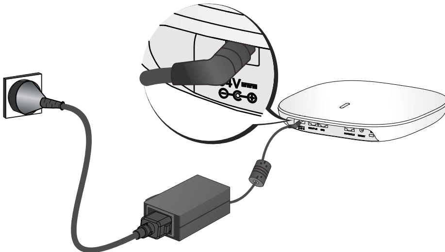
Figure 16 Connecting the local power supply (1)
