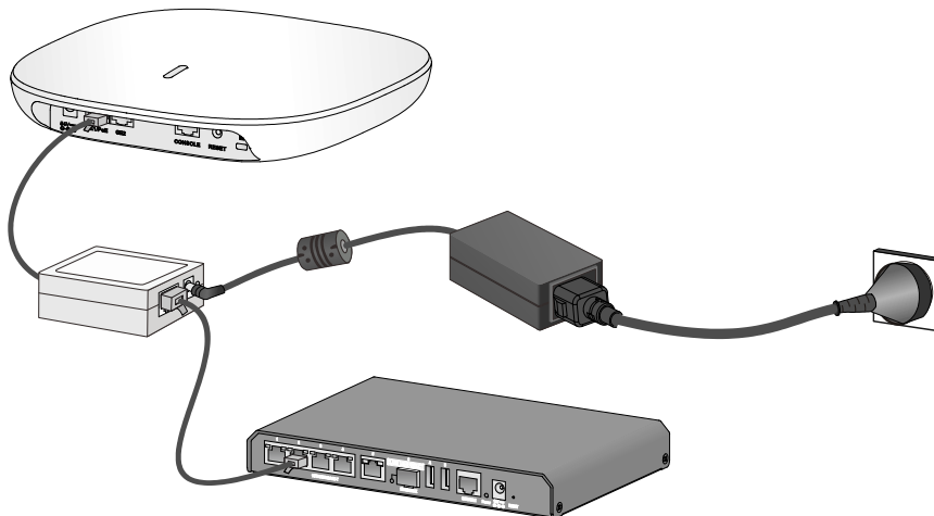
Figure 18 PoE injector power supply
