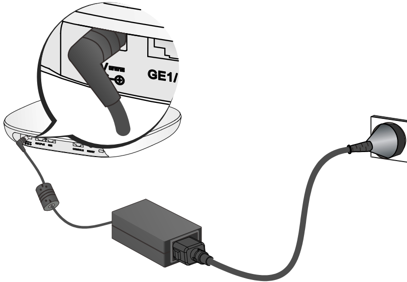
Figure 17 Connecting the local power supply
