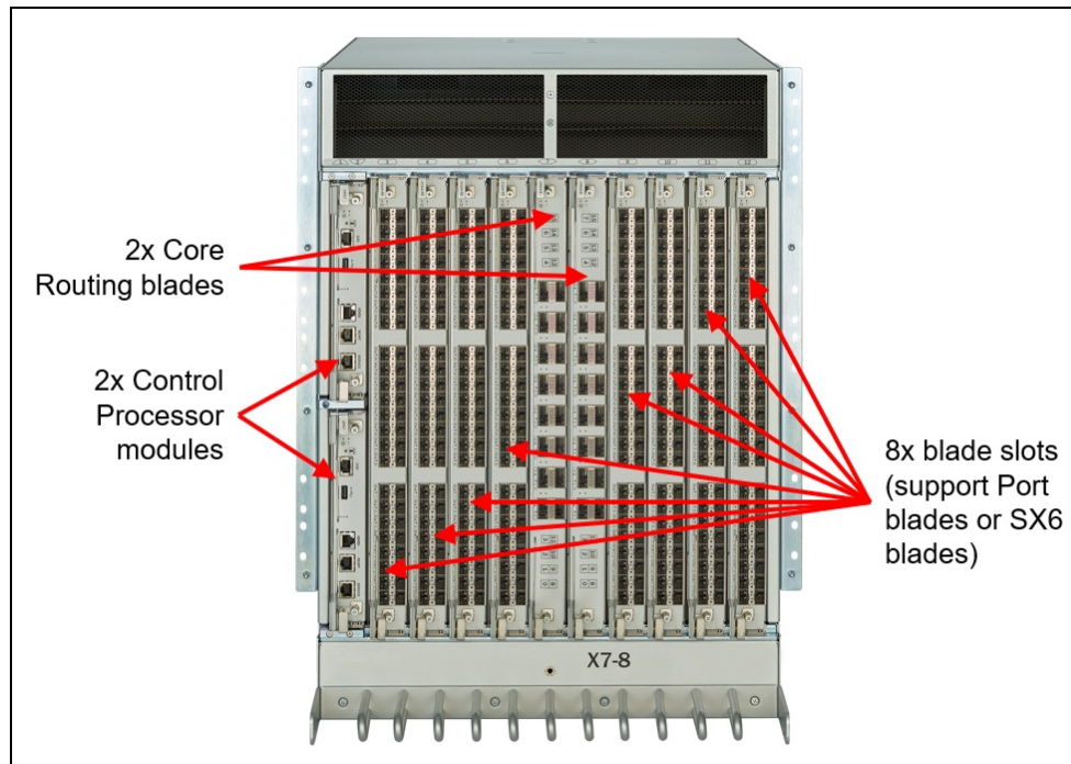
Figure 4. X7-8 FC SAN Director port-side view
