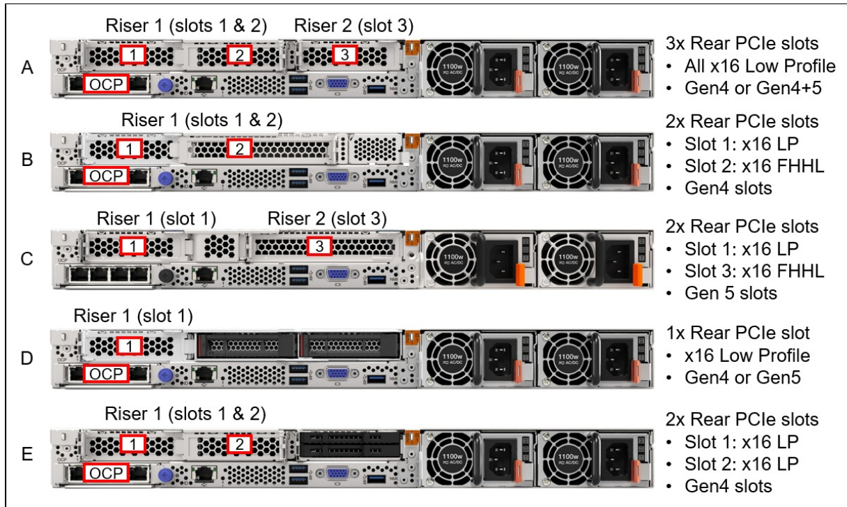
Figure 11. SR635 V3 slot configurations
