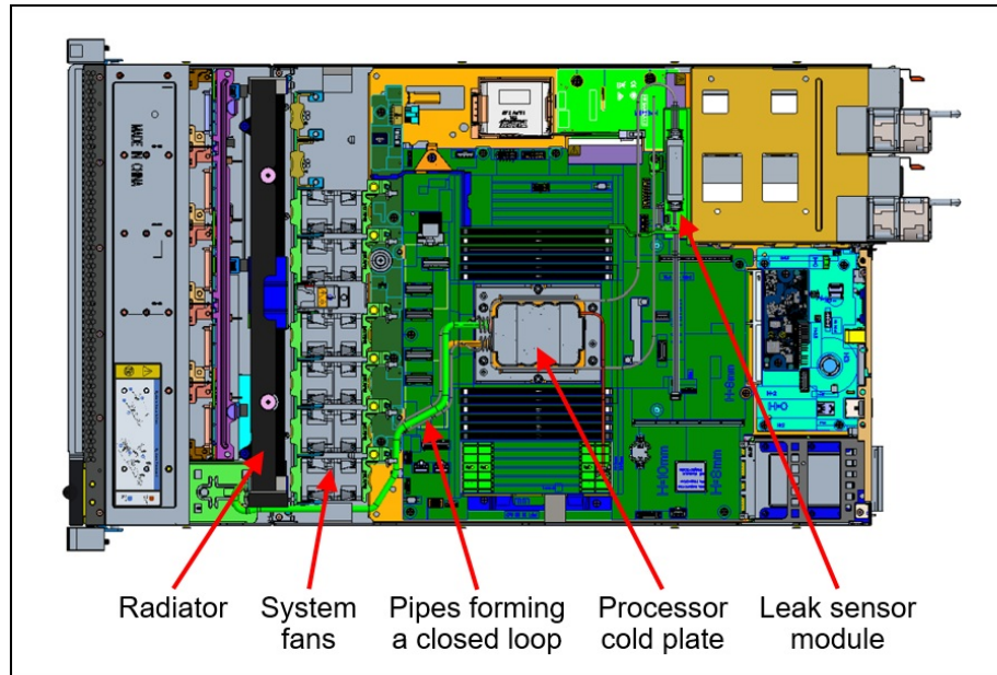
Figure 6. SR635 V3 with closed loop heatsink (feature BS34)
