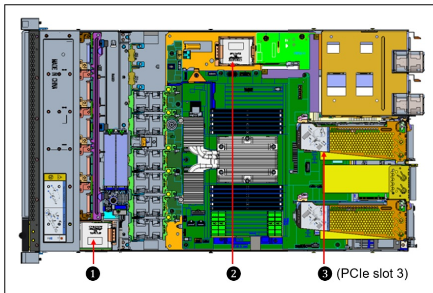
Figure 10. Location of the supercaps in the SR635 V3
