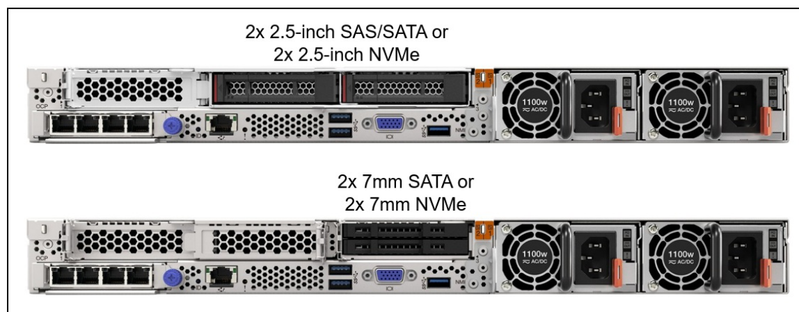
Figure 9. Rear drive bay configurations
