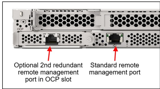
Figure 19. SR635 V3 with the Redundant System Management Port Adapter installed
