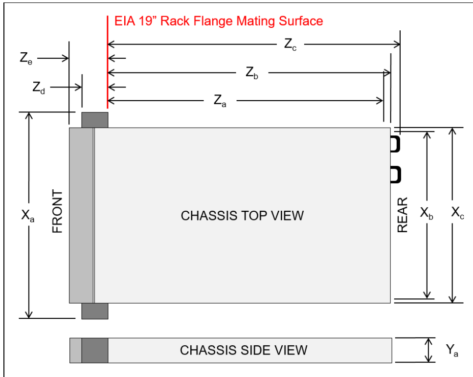
Figure 21. Server dimensions
