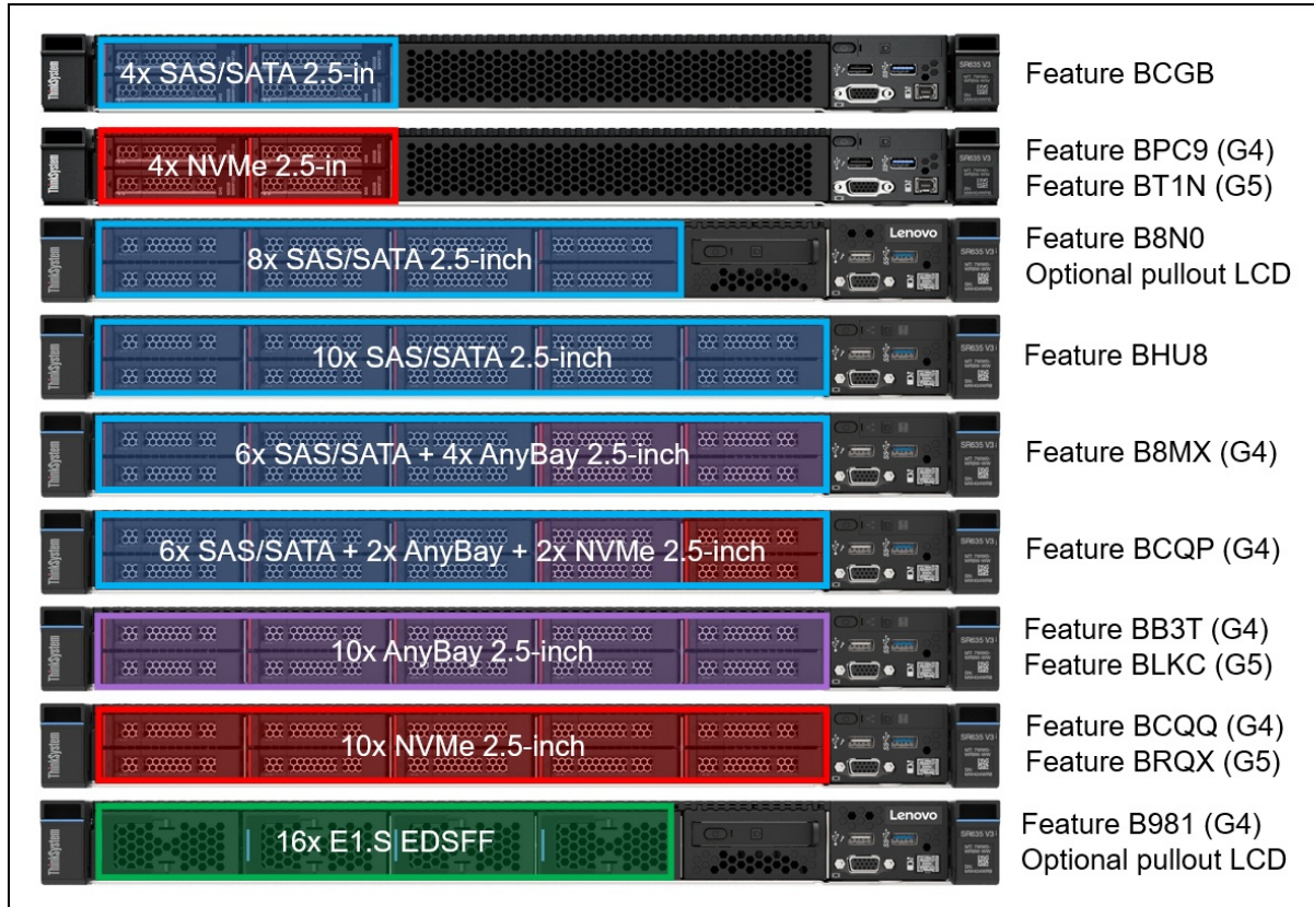
Figure 7. SR635 V3 front drive bay configurations without front PCIe slots
