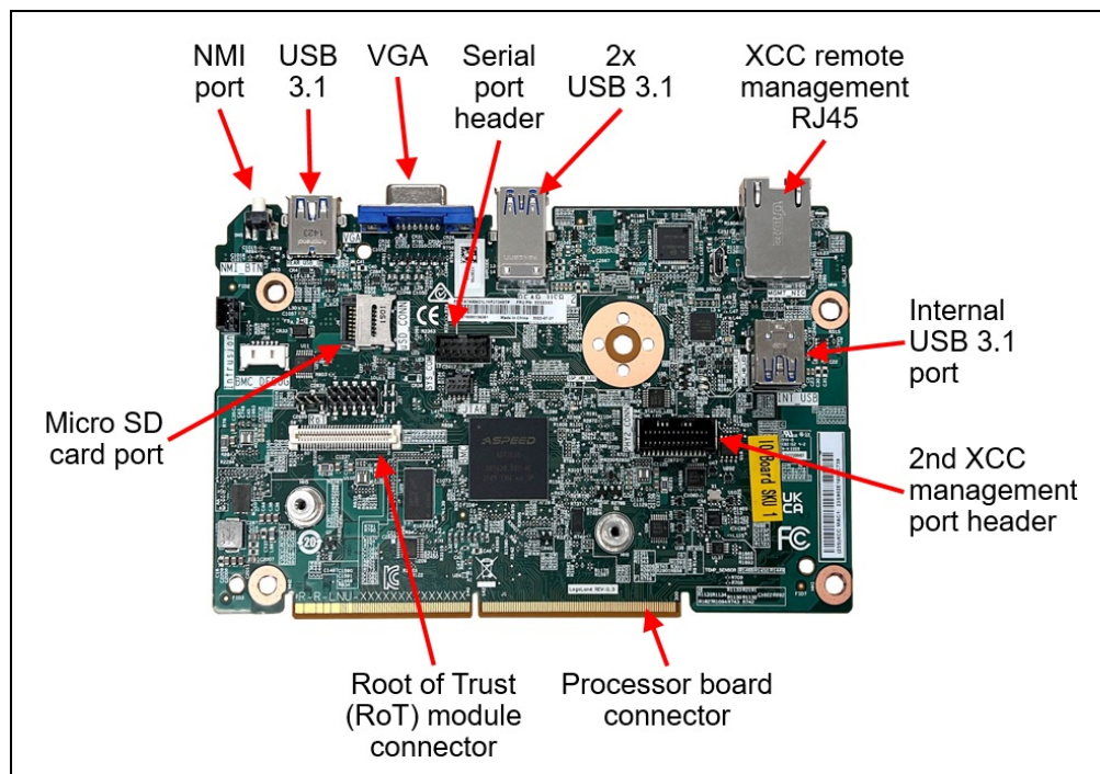
Figure 15. System I/O Board
