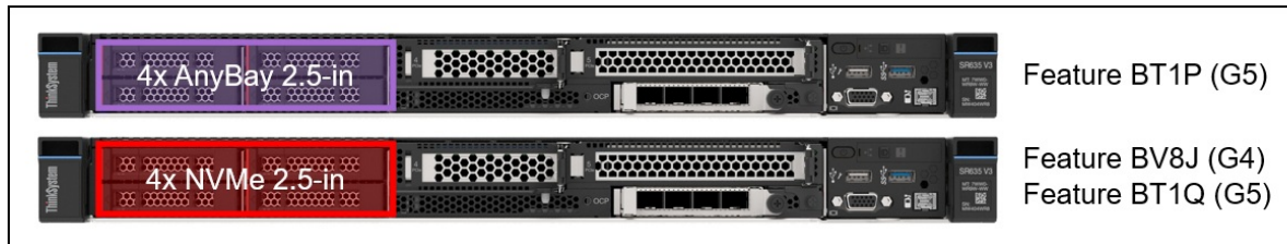
Figure 8. SR635 V3 front drive bay configurations with front PCIe slots
