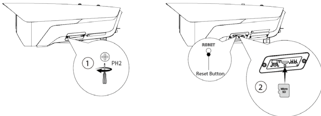
Figure 3-4 Install SD card
