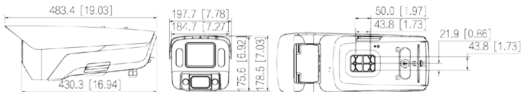
Figure 3-2 Dimensions (mm [inch])
