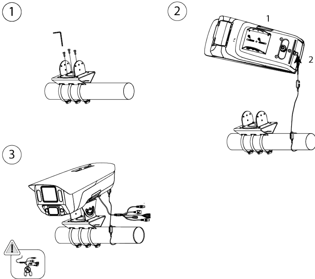
Figure 3-5 Attach camera
