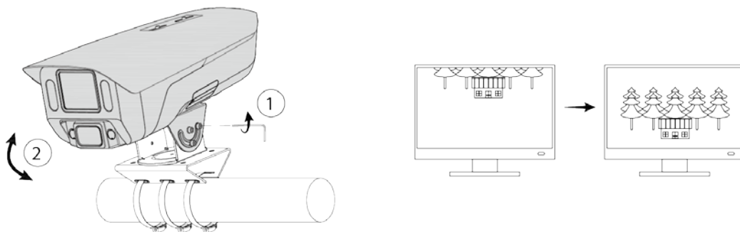
Figure 3-8 Adjust lens angle
