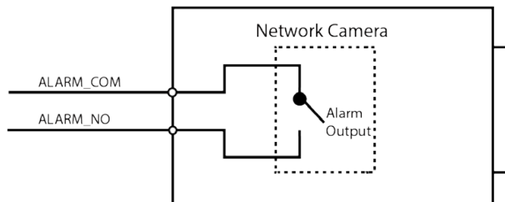
Figure 1-4 Alarm output
