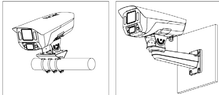
Figure 3-3 Installation method
