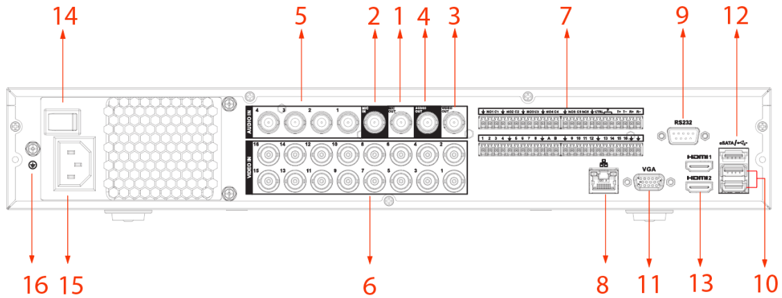
Figure 3-20 Rear panel (3)
