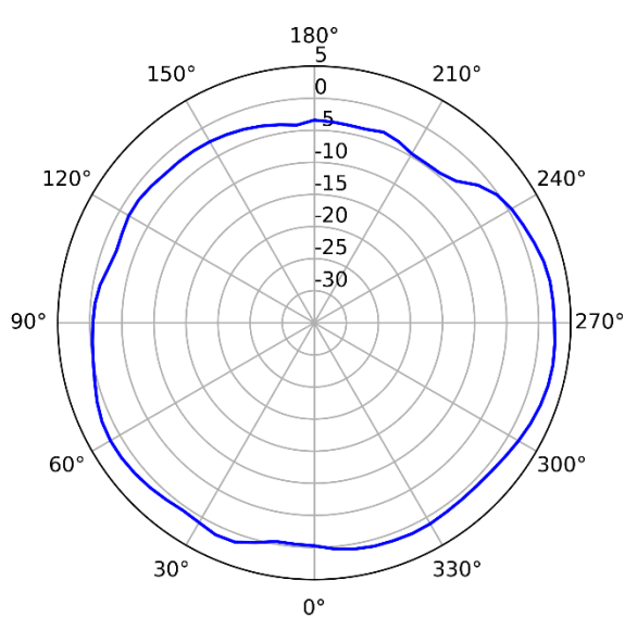
2.4GHz (Horizontal)
