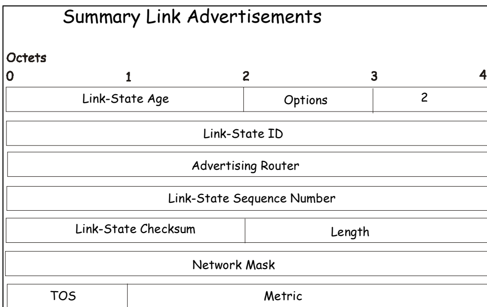
Figure 6-39 Summary Link Advertisements
