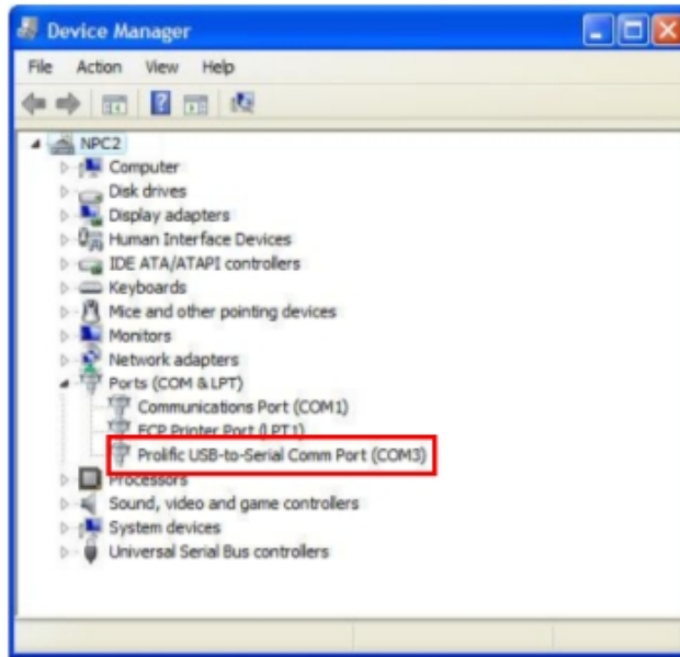
Figure 15 — Device Manager
