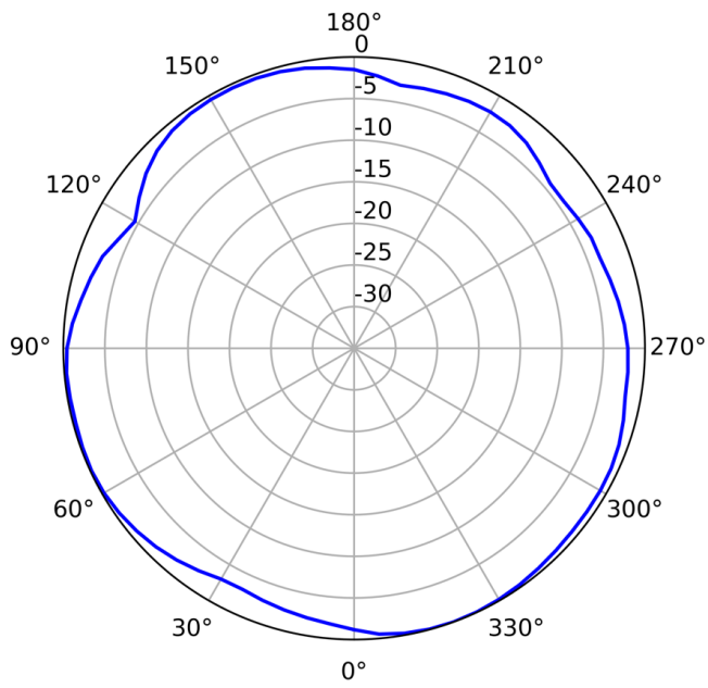
2.4GHz (Horizontal)
