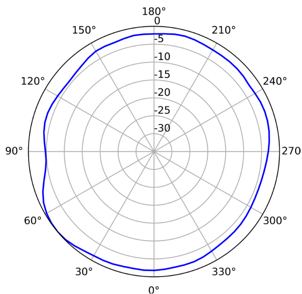
2.4G (Horizontal)
