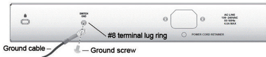
Figure 2.7 – Connect a Grounding Cable
