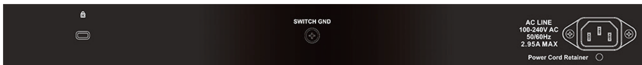
Figure 1.6 – DES-1210-28P Rear Panel
