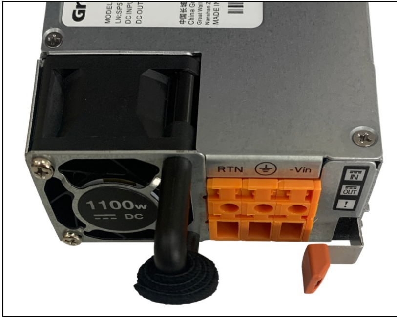
Figure 16. Connector on the ThinkSystem 1100W -48V DC Hot-Swap Gen2 Power Supply
