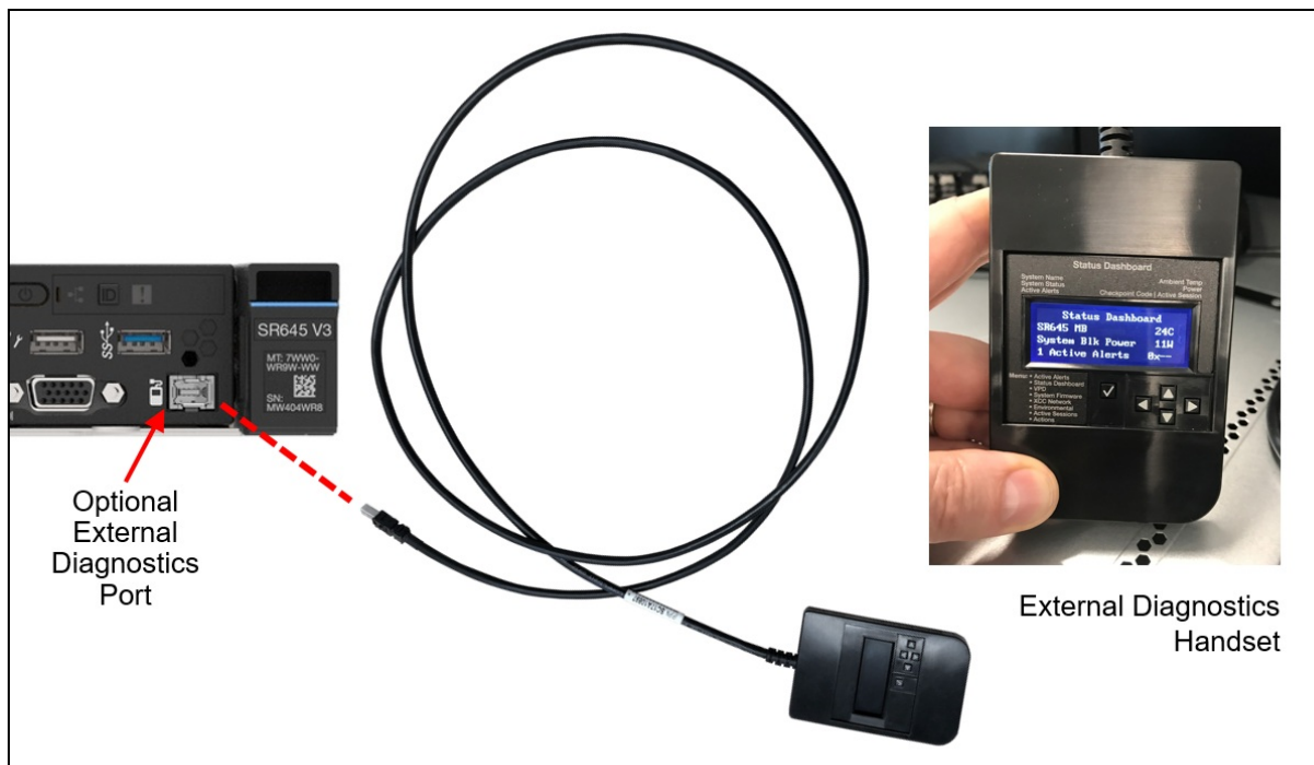
Figure 20. External Diagnostics Handset
