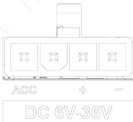
Figure 2-4 Power input interface
