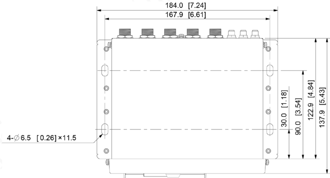
Figure 2-8 Lug installation dimensions (mm [inch])
