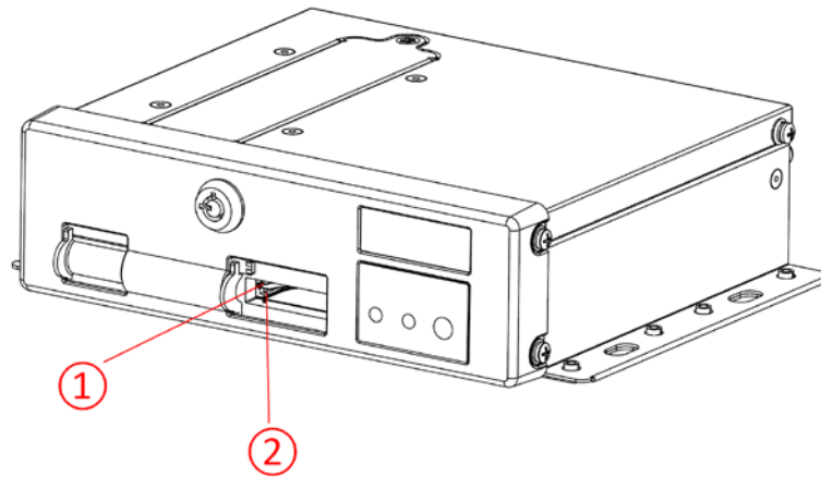
Figure 2-12 Install SD card (SSD version)
