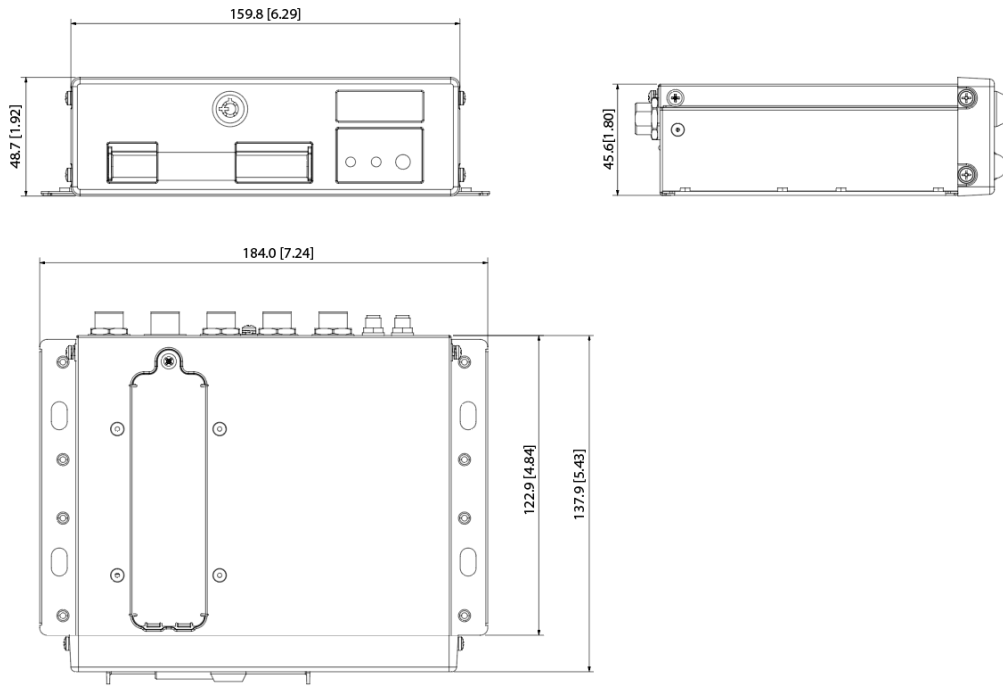
Figure 2-10 Lug installation dimensions (SSD version) (mm [inch])
