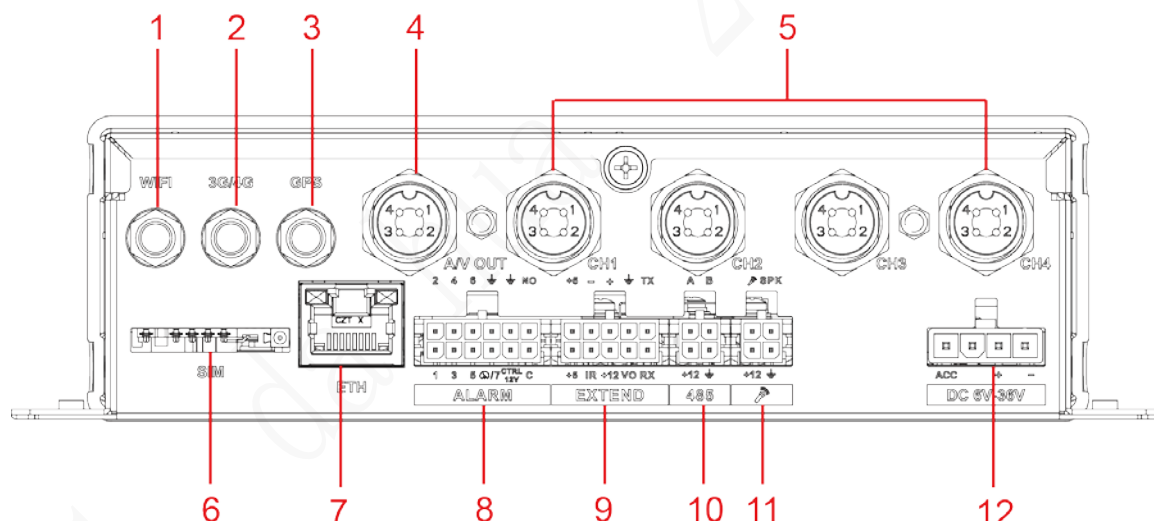
Figure 2-2 Rear Panel
