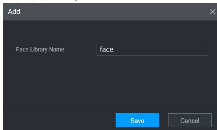
Figure 5-14 Add
