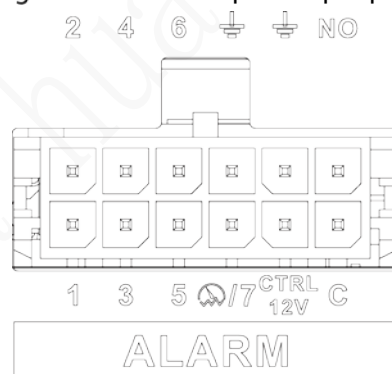
Figure 2-27 Alarm input/output port
