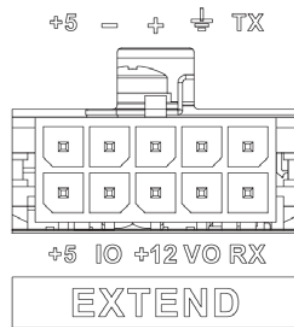
Figure 2-5 EXTEND port
