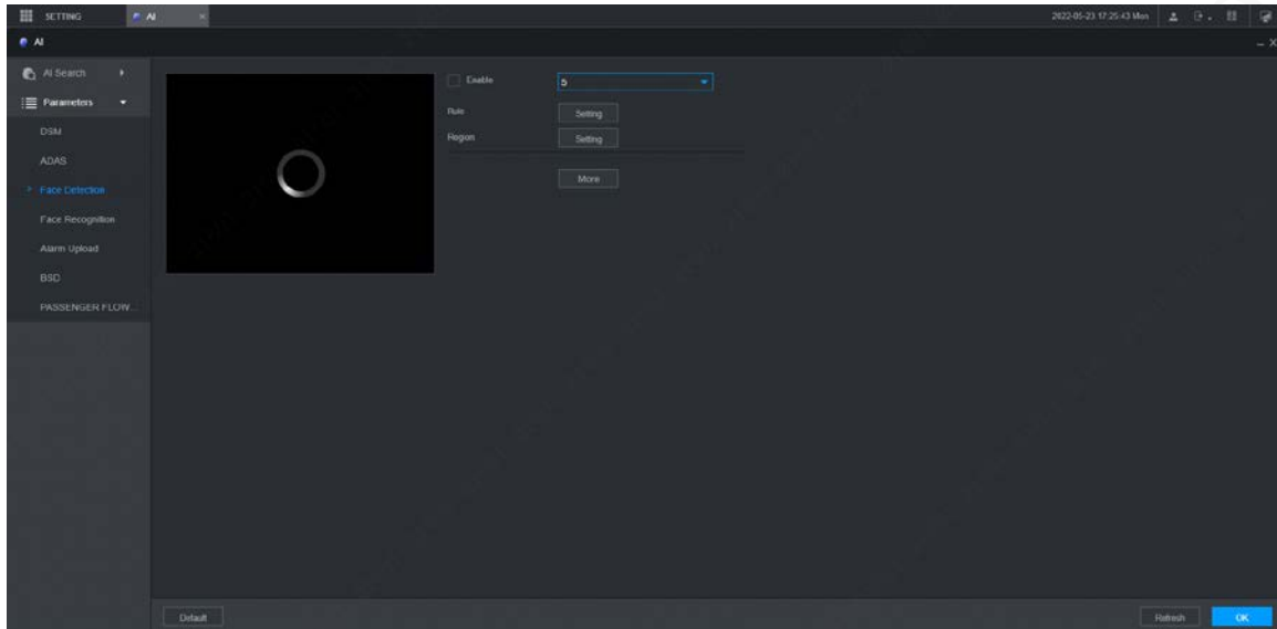
Figure 5-10 Face detection
