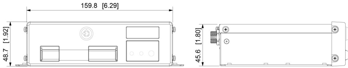
Figure 2-7 Physical Dimensions (mm [inch])
