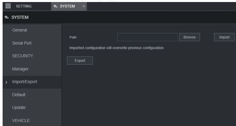
Figure 7-10 Configuration import/export (2)
