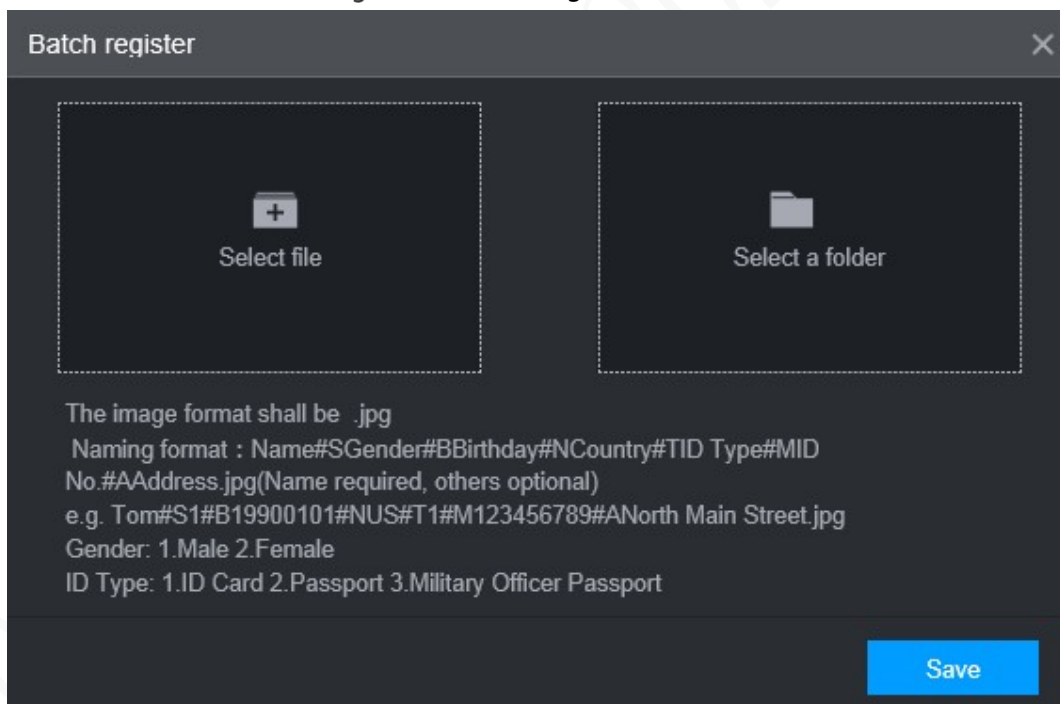
Figure 5-20 Batch register
