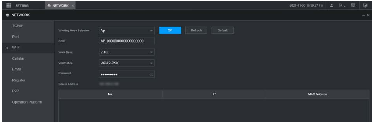
Figure 5-43 Ap settings
