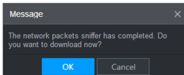
Figure 7-15 Prompt
