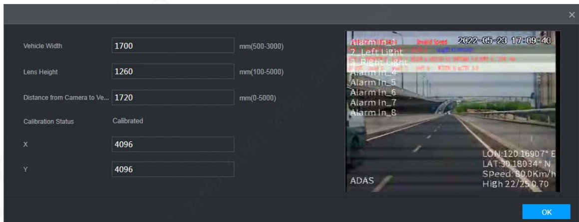
Figure 5-9 Calibration
