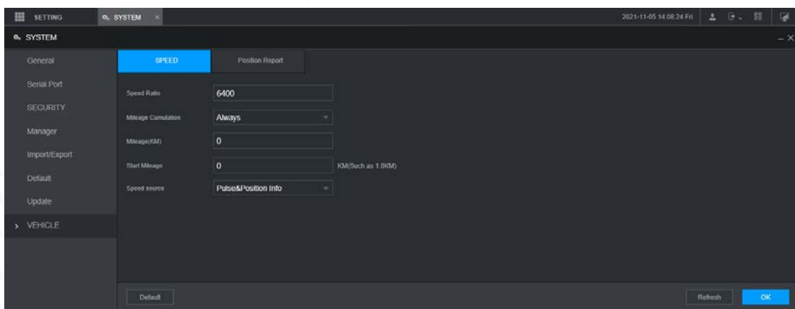
Figure 5-54 Speed
