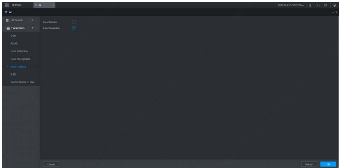
Figure 5-26 Alarm Upload
