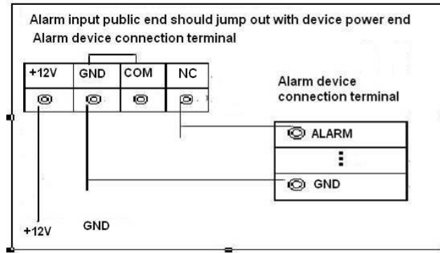
Figure 2-28 Normal Closed alarm input illustration
