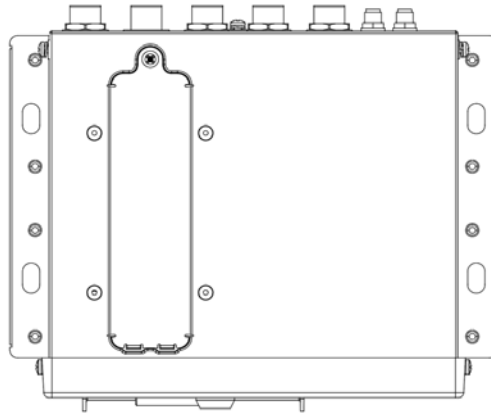
Figure 2-22 Fix the Device onto the vehicle. (SSD version)
