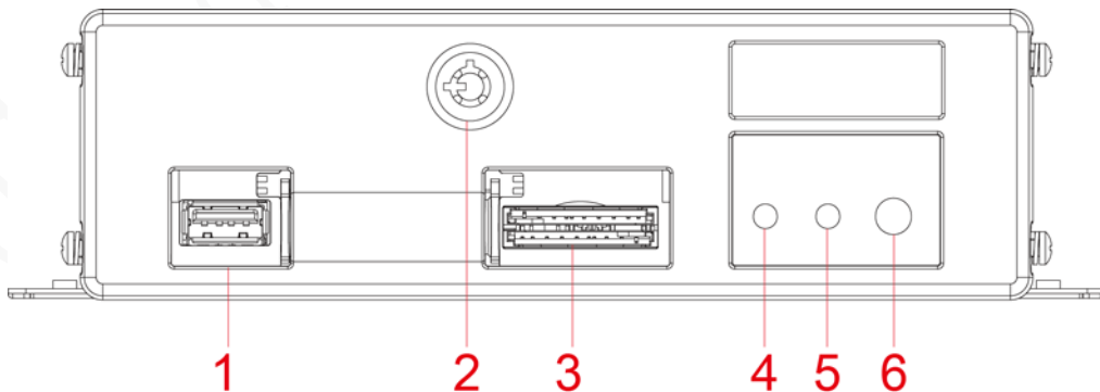
Figure 2-1 Front Panel
