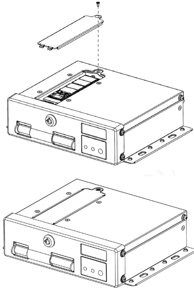
Figure 2-16 Install slot cover
