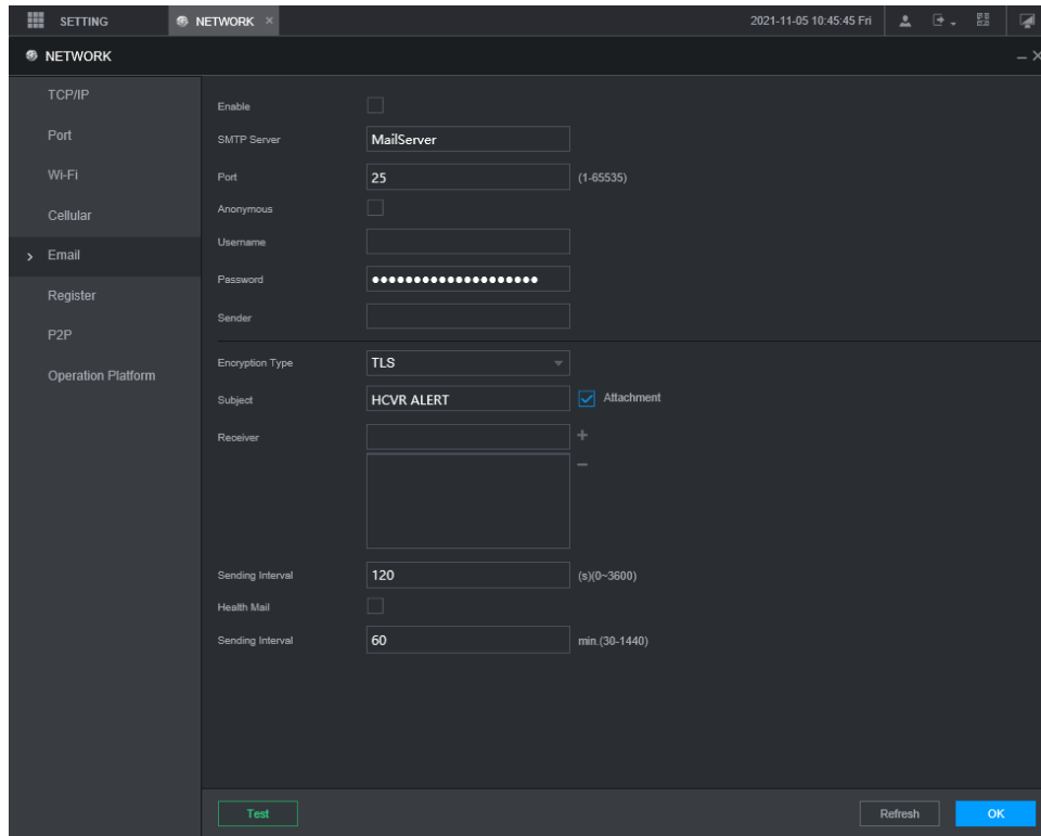
Figure 5-45 Email settings
