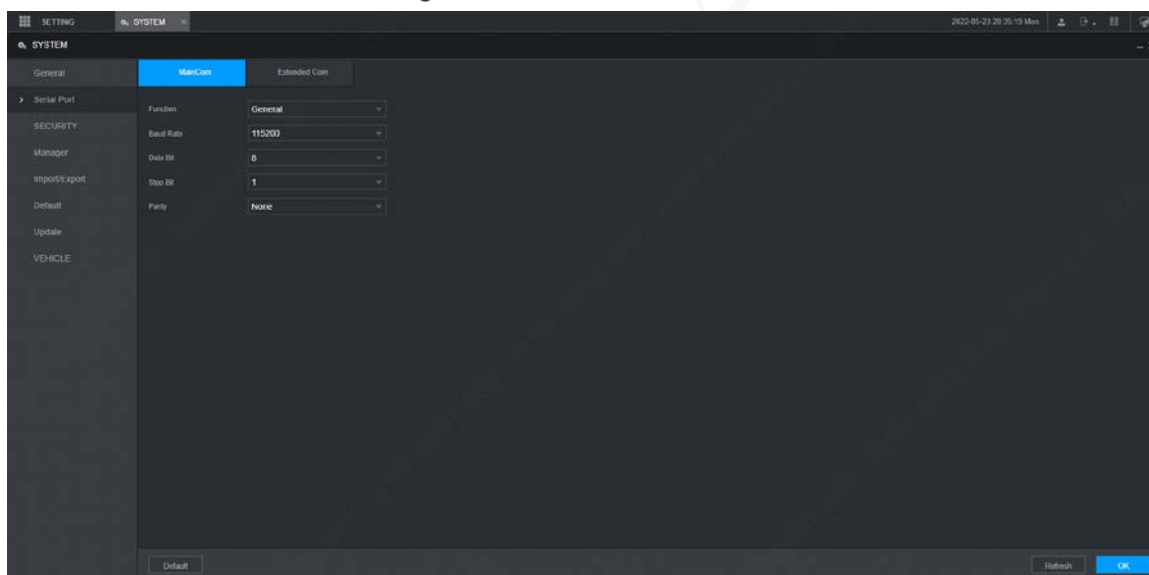
Figure 5-57 Serial Port
