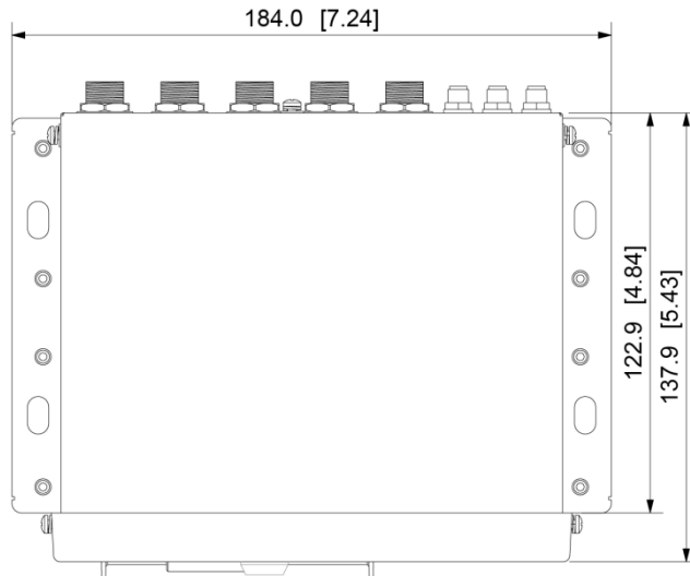
Figure 2-8 Lug installation dimensions (mm [inch])
