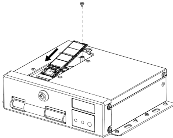
Figure 2-15 Install SSD
