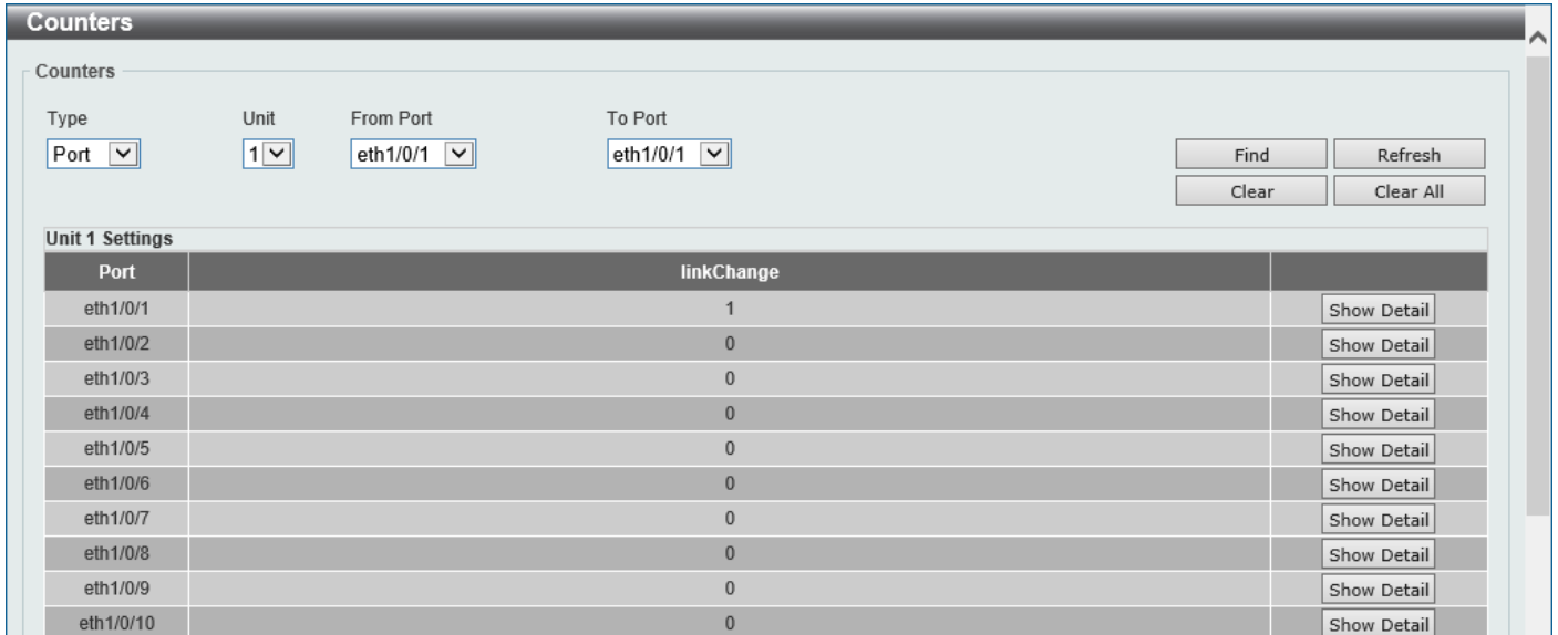
Figure 13-13 Counters (Port) Window
