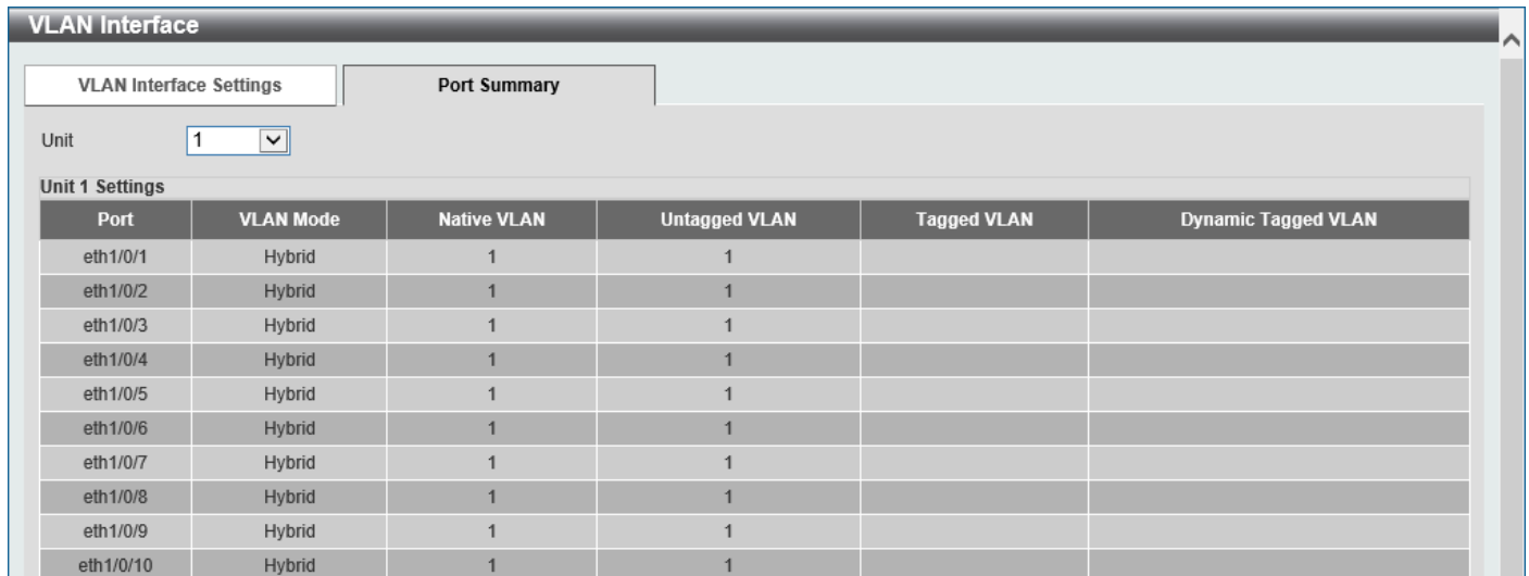
Figure 5-18 Port Summary Window
