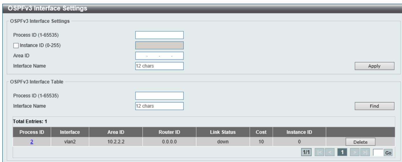
Figure 6-76 OSPFv3 Interface Settings Window
