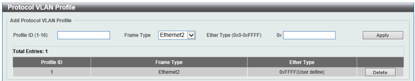
Figure 5-19 Protocol VLAN Profile Window
