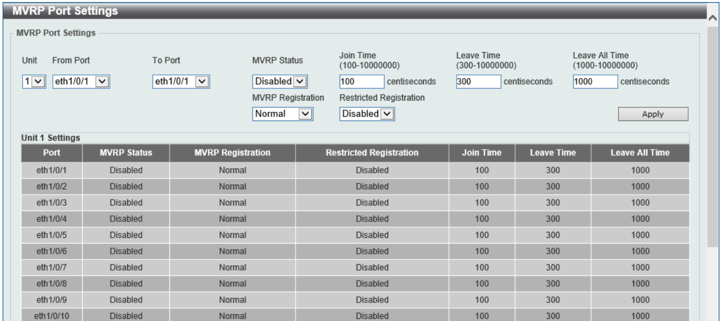
Figure 5-27 MVRP Port Settings Window
