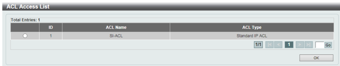
Figure 6-91 IGMP SSM Mapping Settings (Select) Window
