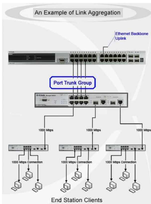
Figure 5-65 Example of Port Trunk Group
