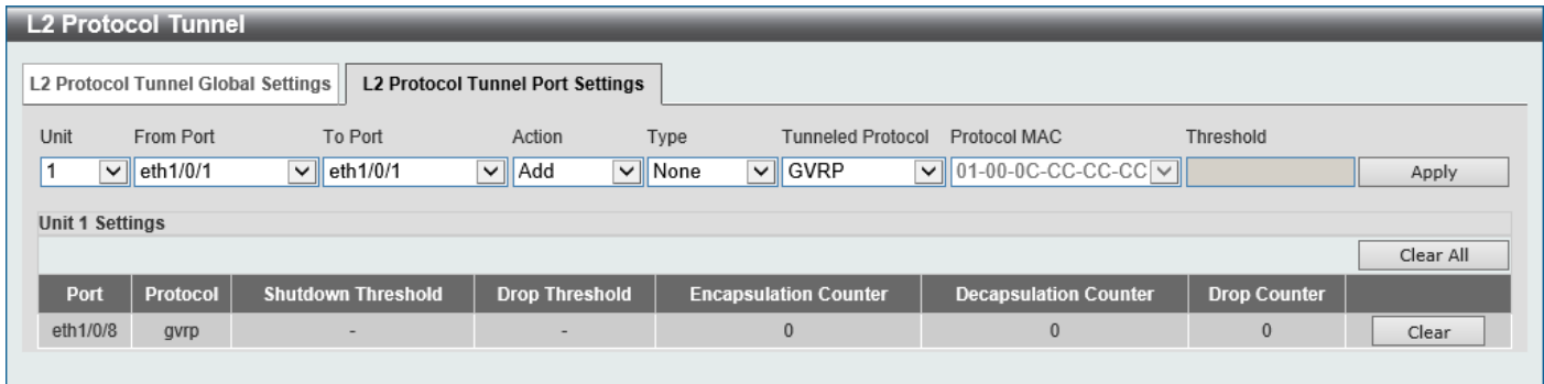
Figure 5-73 L2 Protocol Tunnel (L2 Protocol Tunnel Port Setting) Window
