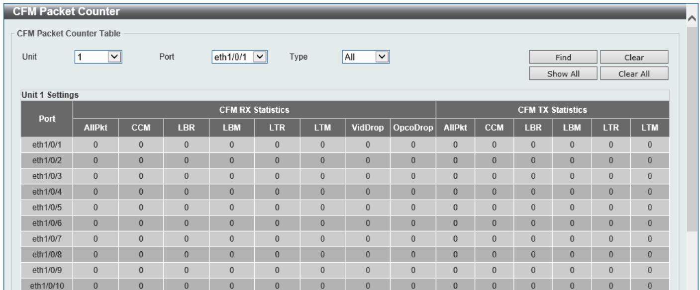
Figure 10-15 CFM Packet Counter Window
