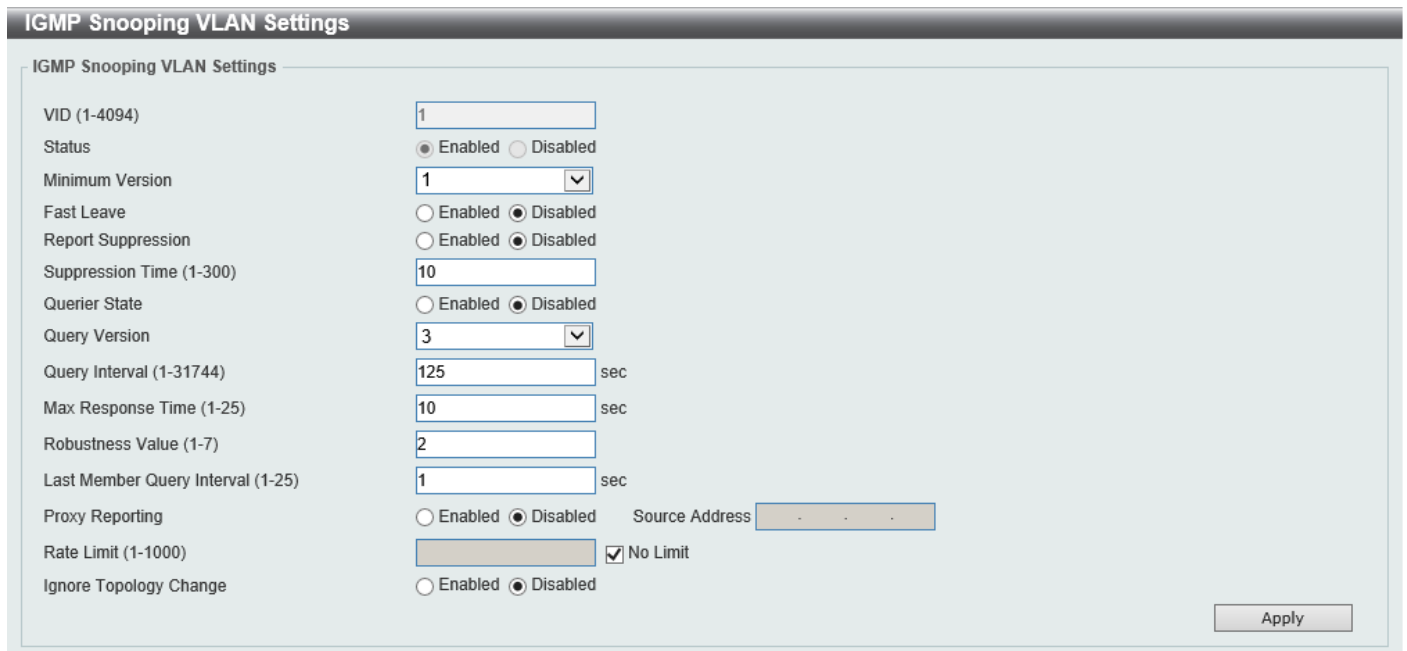
Figure 5-76 IGMP Snooping Settings (Modify, Edit) Window
