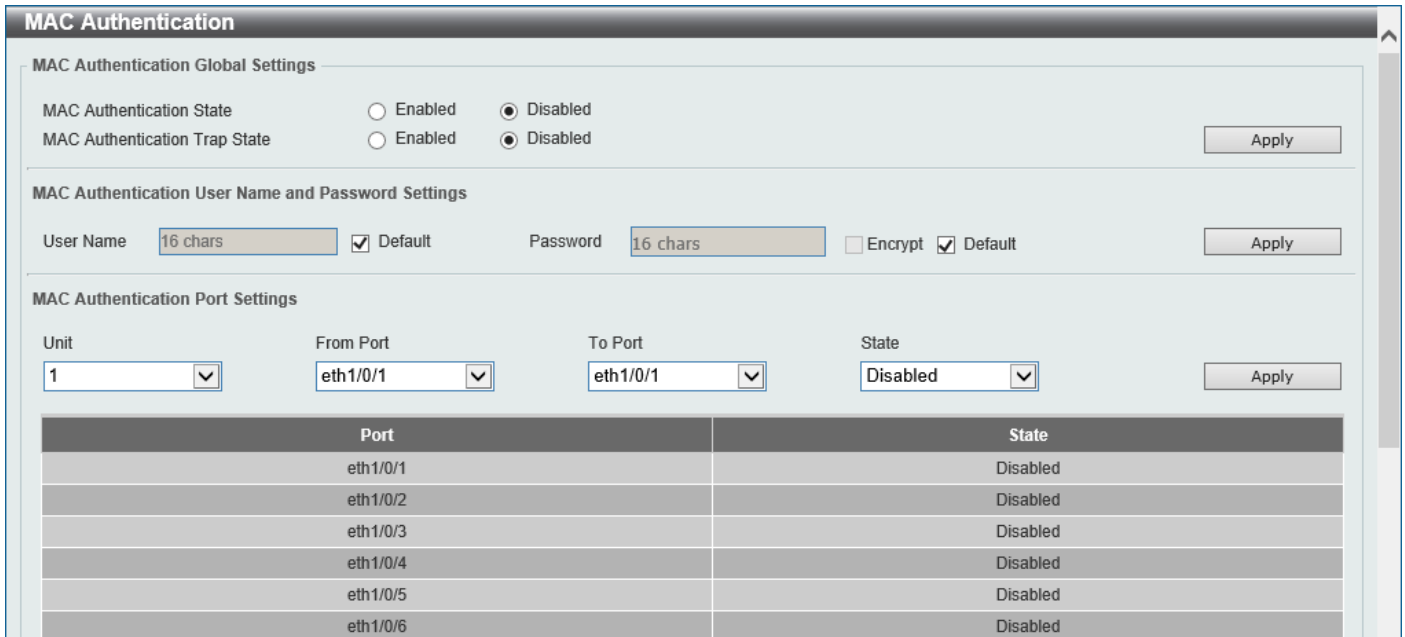
Figure 9-70 MAC Authentication Window
