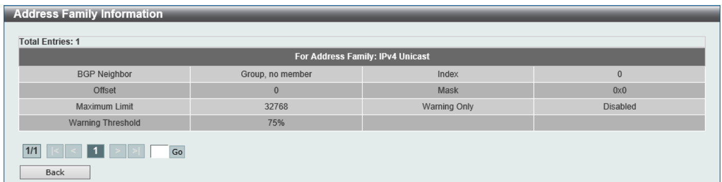
Figure 6-192 Peer Group (Show Detail) Window
