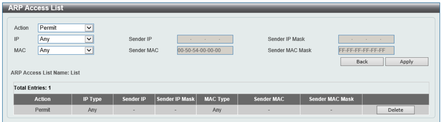
Figure 9-45 ARP Access List (Edit) Window
