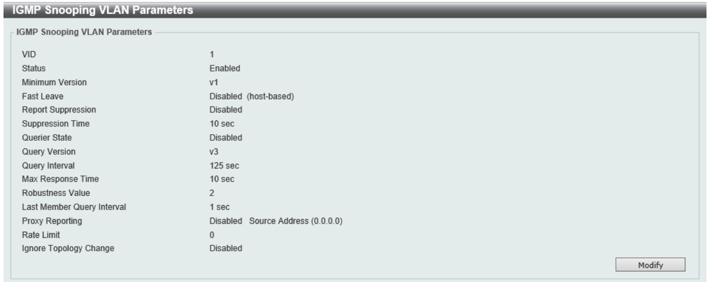
Figure 5-75 IGMP Snooping Settings (Show Detail) Window
