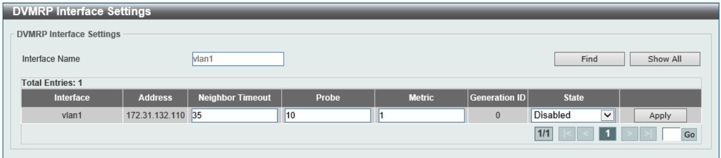
Figure 6-105 DVMRP Interface Settings (Edit) Window
