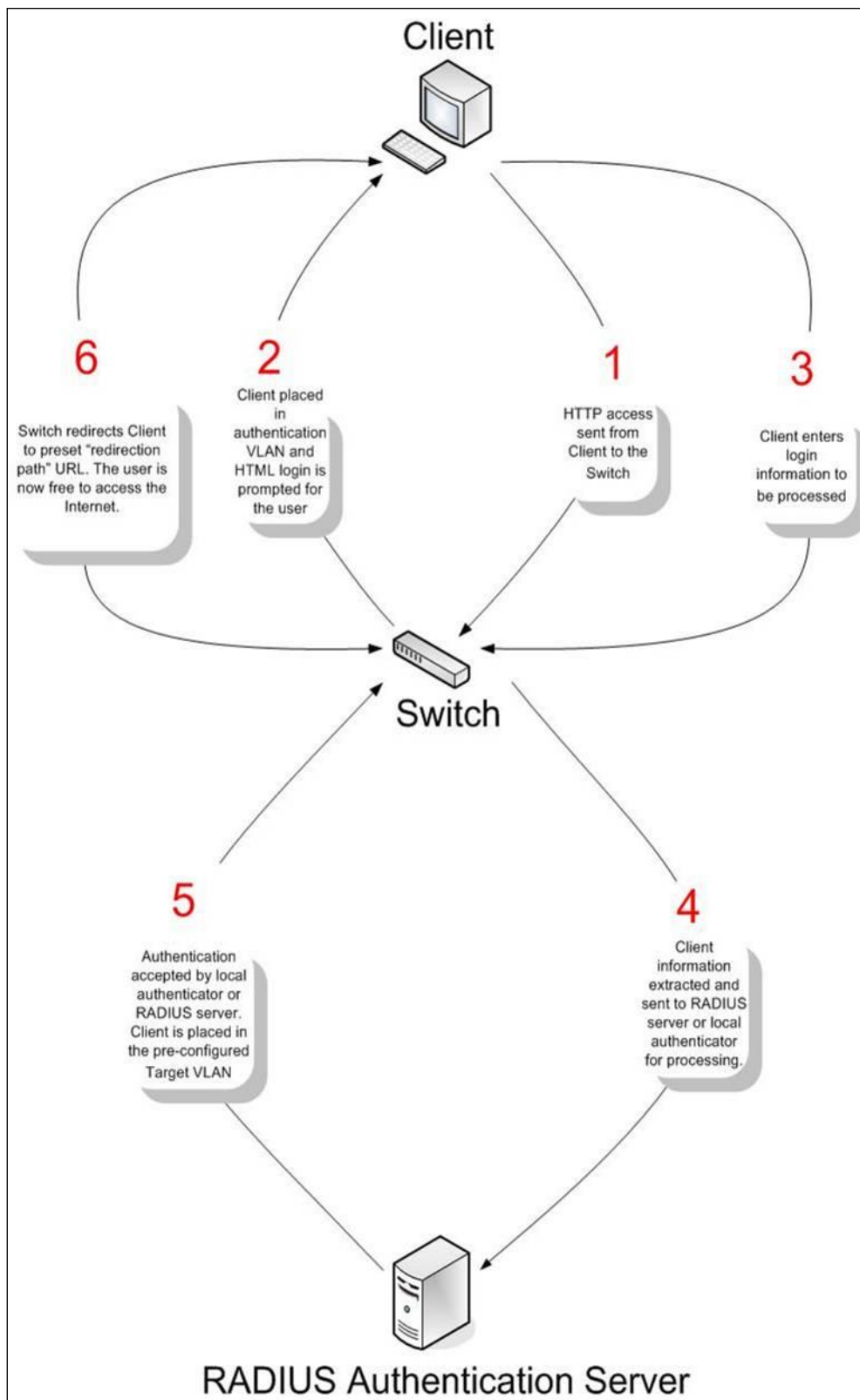
Figure 9-71 RADIUS Authentication Server
