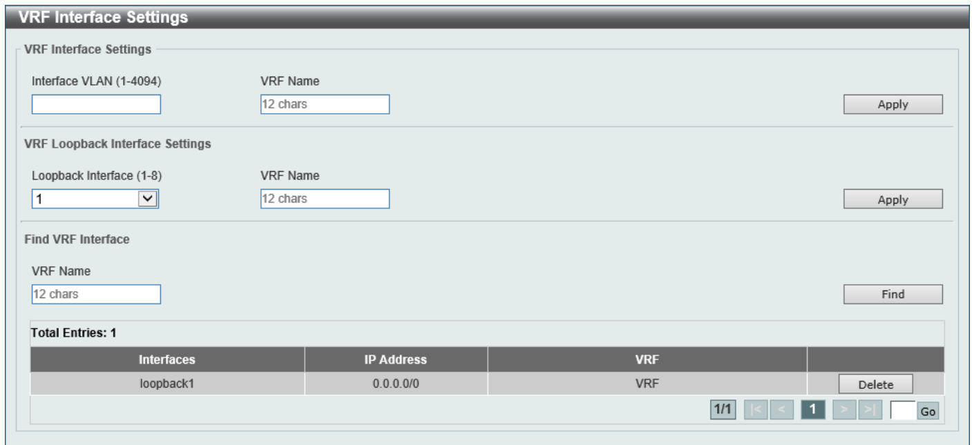
Figure 6-38 VRF Interface Settings Window
