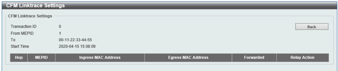
Figure 10-14 CFM Linktrace Settings (Show Detail) Window
