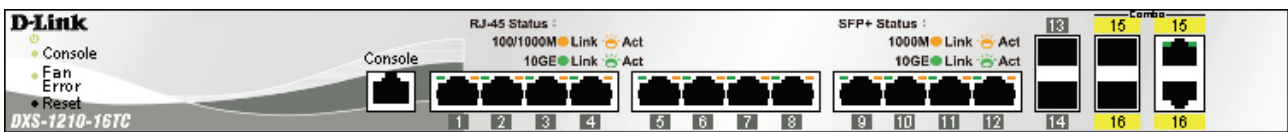
Figure 1.7 – DXS-1210-16TC Front Panel
