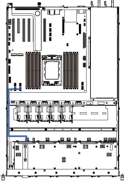
U.2 NVMe to HDD Back Plane Board Cable (NVMe1)
