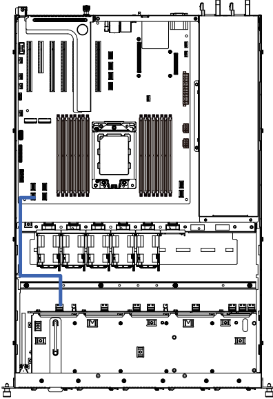
U.2 NVMe to HDD Back Plane Board Cable (NVMe0)
