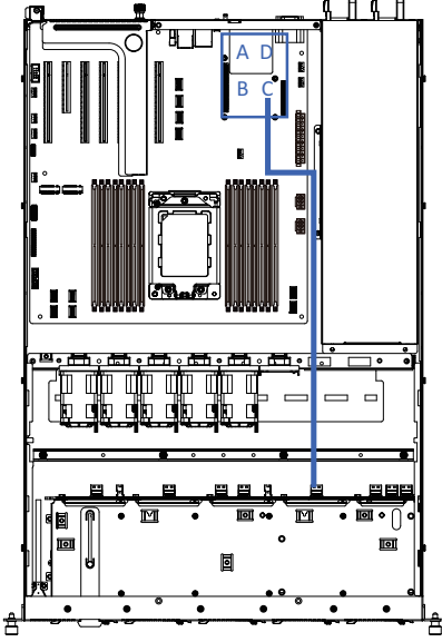
U.2 NVMe to HDD Back Plane Board Cable (NVMe6)
