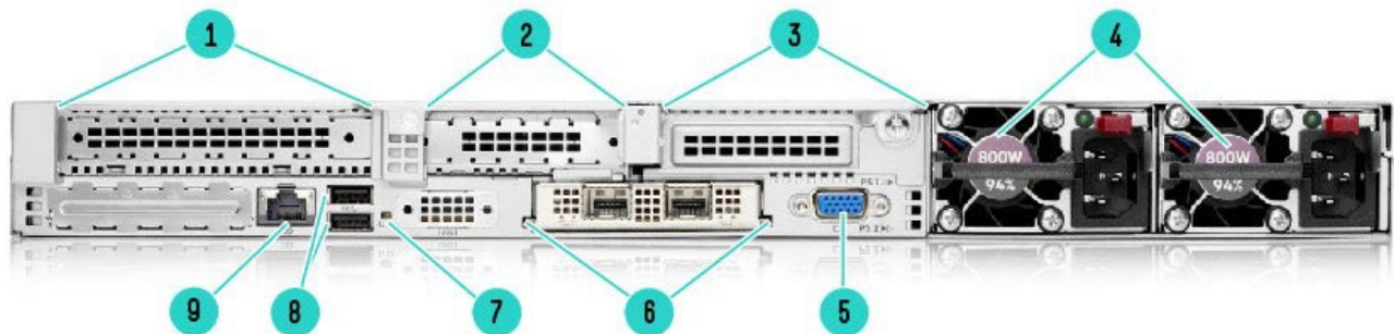
Rear View – Standard for all DL365 Gen10 Plus
