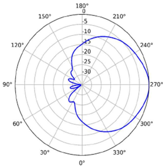
2.4GHz (Horizontal)
