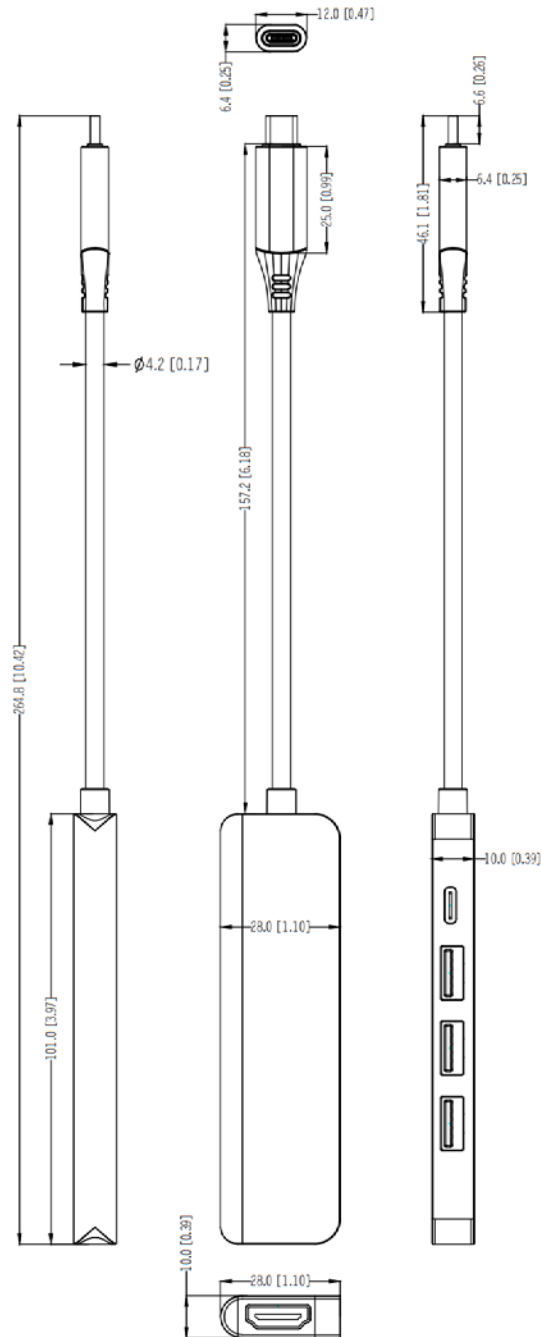
Figure 1-1 Dimensions (Unit: mm [inch])
