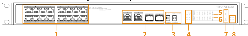
Figure 2-1 Front panel
