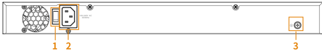
Figure 2-2 Rear panel
