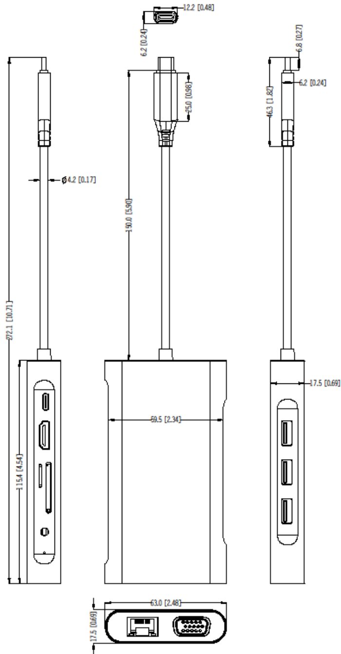
Figure 1-1 Dimensions (Unit: mm [inch])
